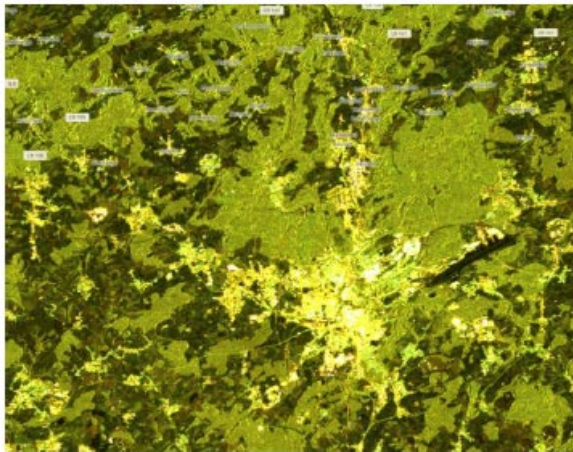
Sentinel 1: (Radarbild)
